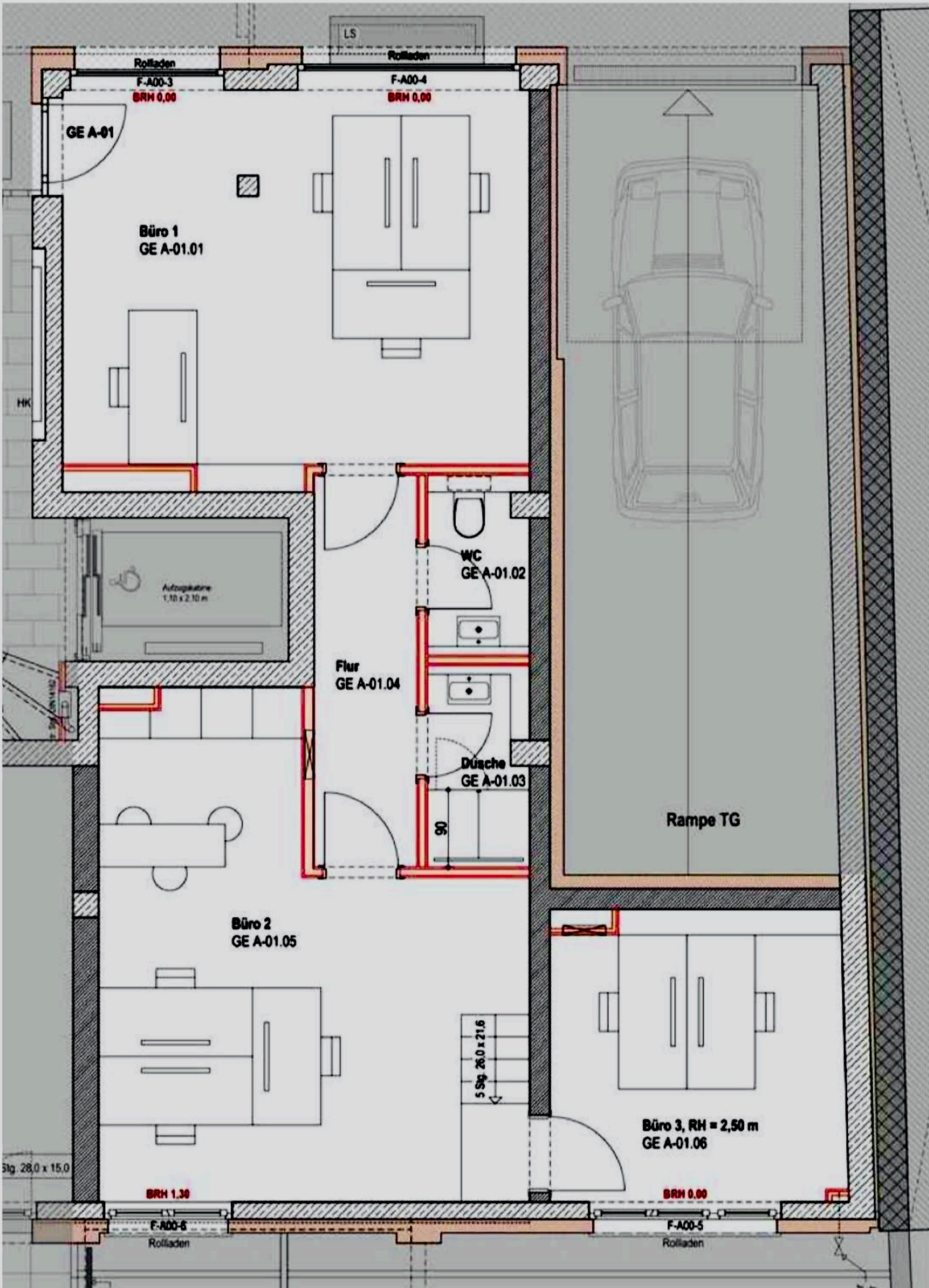
Grundriss_GE 01
